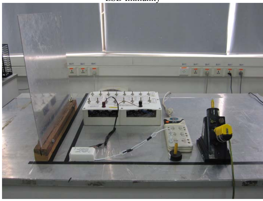
ESD Immunity
