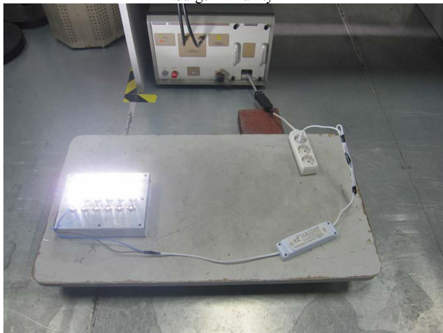
Radiated Electromagnetic Field Disturbance (9kHz-30MHz)
